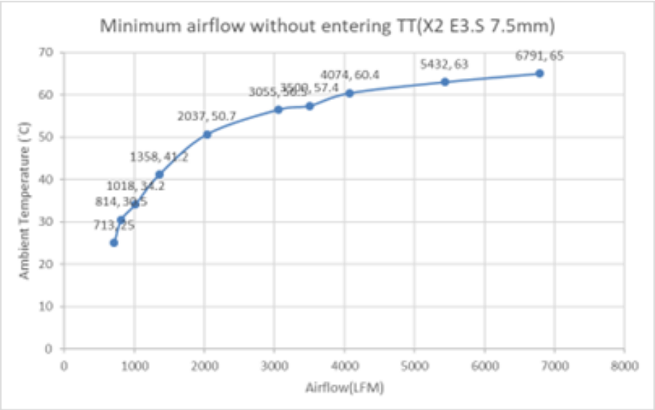
Airflow Profile Chart
